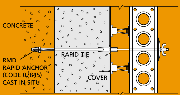
Single Faced Application Using cast in anchor
