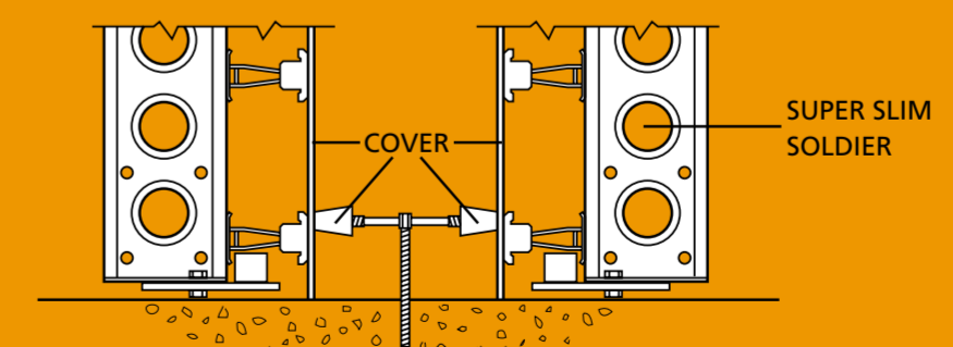
Support Leg (Code 08681). Concrete End Caps (Code 08689). Threaded horizontal bar (Code 08682-08688 and 08691). End caps give 50mm cover threaded bar length determined by wall: all thickness less 100mm.
