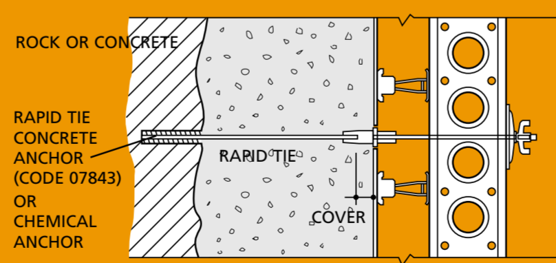
Single Faced Application Using mechanical or chemical anchor into existing face
