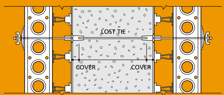
Double Faced Application Cover, either 50mm (Code 07832) or 75mm (Code 07834) Lost Tie is 15mm Rapid Bar Tie (cut to suit)
